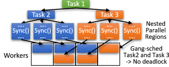
(b) Deadlock avoidance with gang-scheduling of nested parallel tasks
