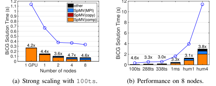
Fig. 11. Performance on Reedbush-H. The blue markers show the solution time with original HACApK without GPUs, while the bars are with the GPUs.
